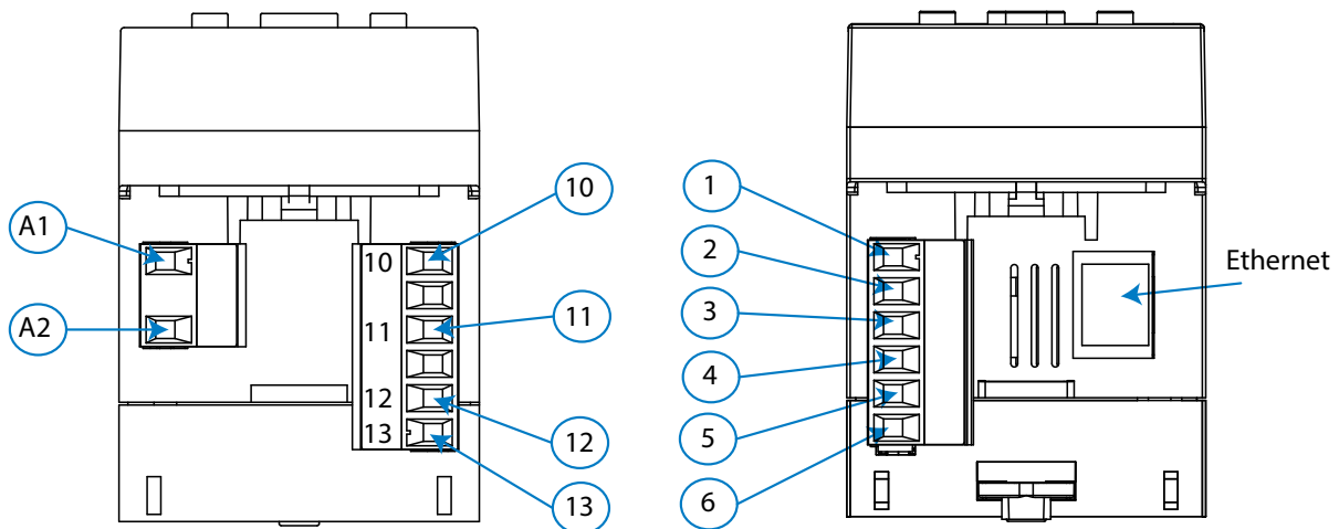
Figura 5: Bornes del CVM-E3-MINI-ITF/MC/FLEX-WiEth: Superior - Inferior.
