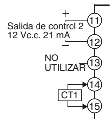
E53-CN03N2
