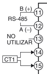
E53-CN03N2
