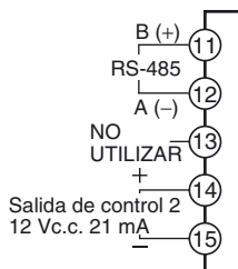
E53-CN03N2
