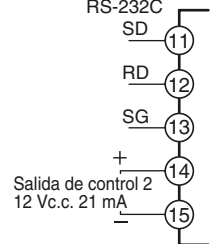
E53-CN03N2
