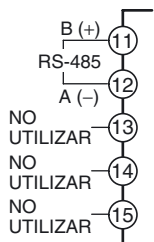
E53-CN03N2
